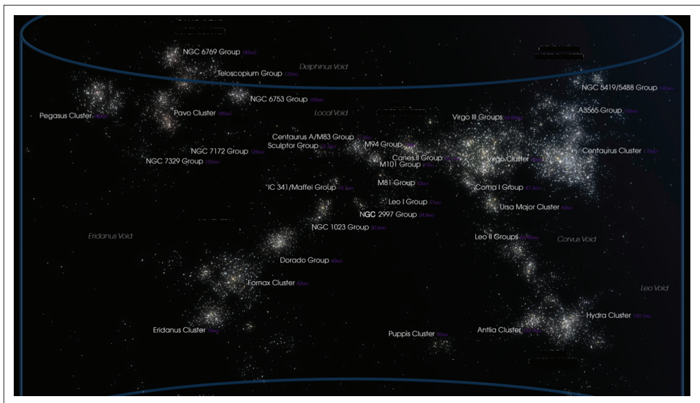
FIGURE 3.4: Map of the galaxy clusters comprising the Laniakea Supercluster.
