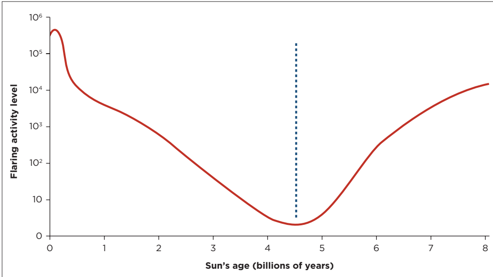
FIGURE 3.1: Sun's level of flaring activity and deadly radiation emission throughout its nuclear burning history.
