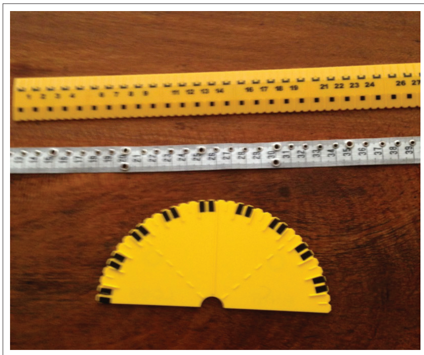
FIGURE 6.8: Measuring equipment for the visually impaired.
